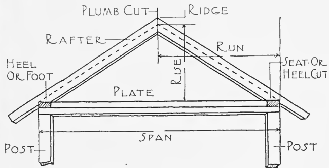
FIG. 29. “RUN” AND “RISE” OF RAFTERS.
